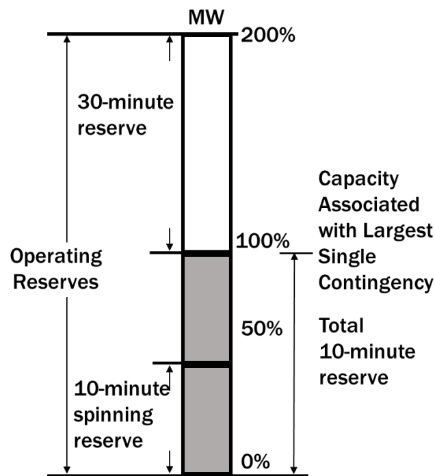
Figure 1112: Minimum Operating Reserve Requirements
