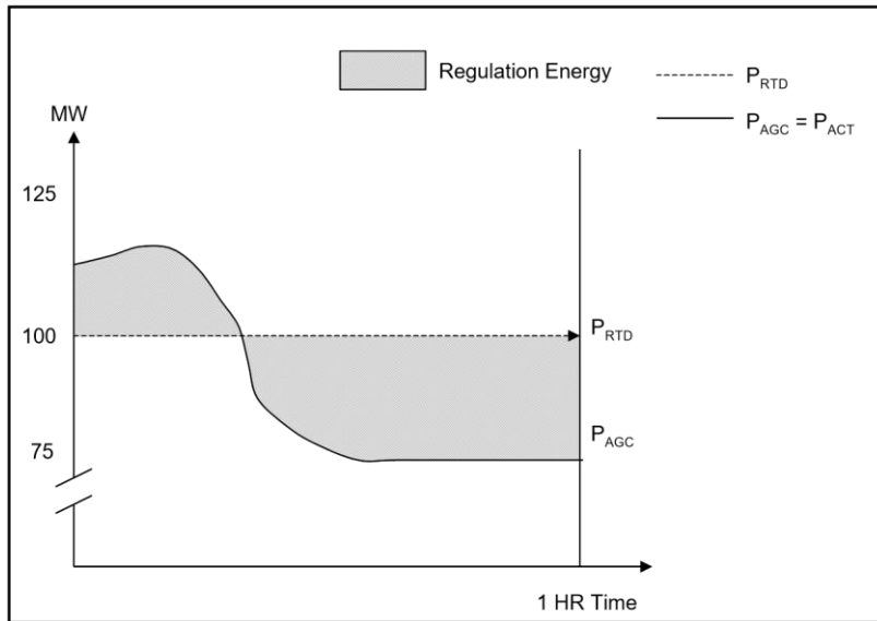
Figure 1011: Error in Performance (30-Second Bandwidth not Included)
