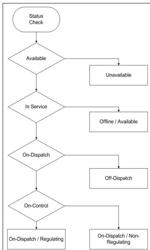
Figure 89: Generating Unit Operating States
