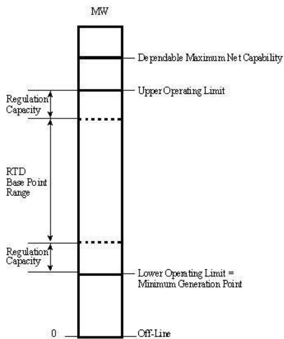
Figure 56: Generating Unit Operating Characteristics
